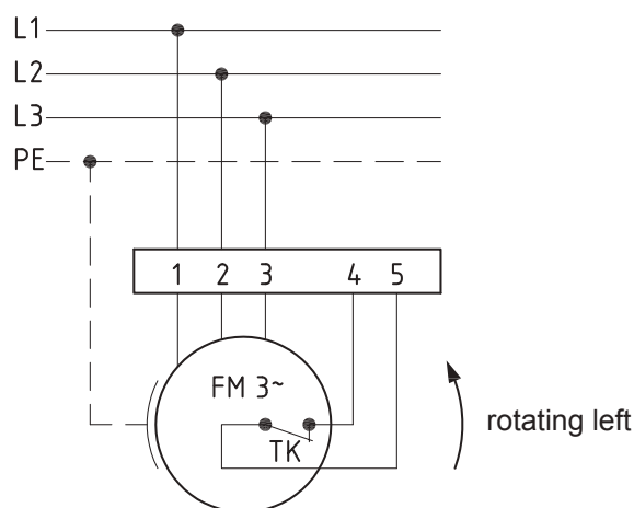
connection plan 0.13-2 I.
