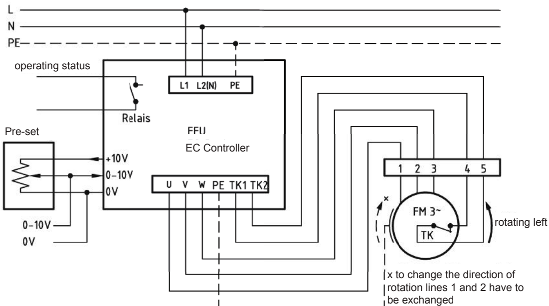
connection plan* FFU-EC 230
