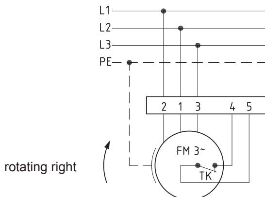
connection plan 0.13-2 r.
