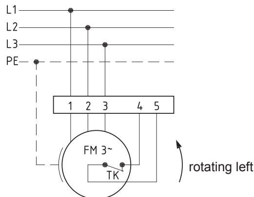
connection plan 0.13-2 l.
